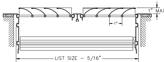
Standard blade option (shown). See following page for other options
