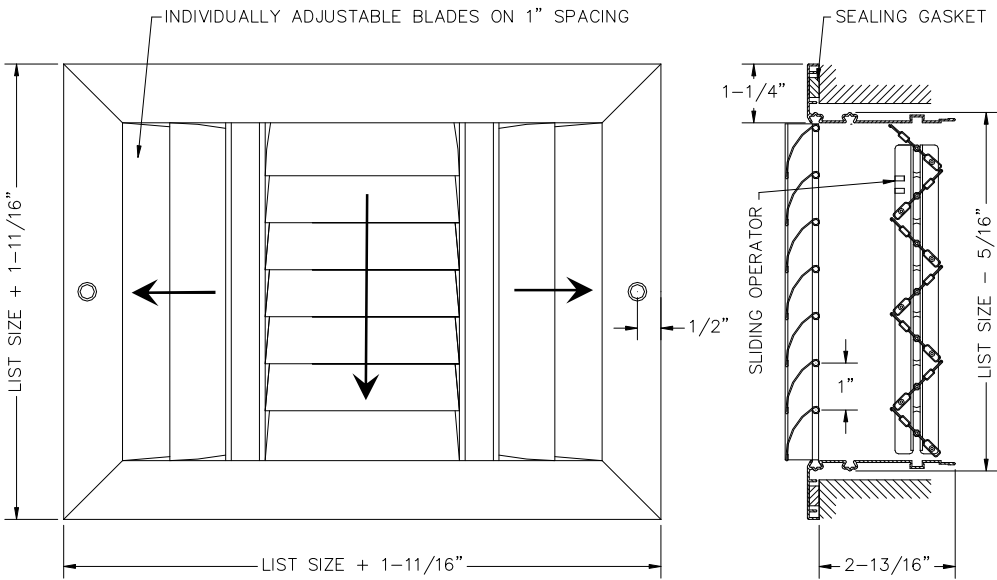
Standard blade option (shown). See following page for other options
